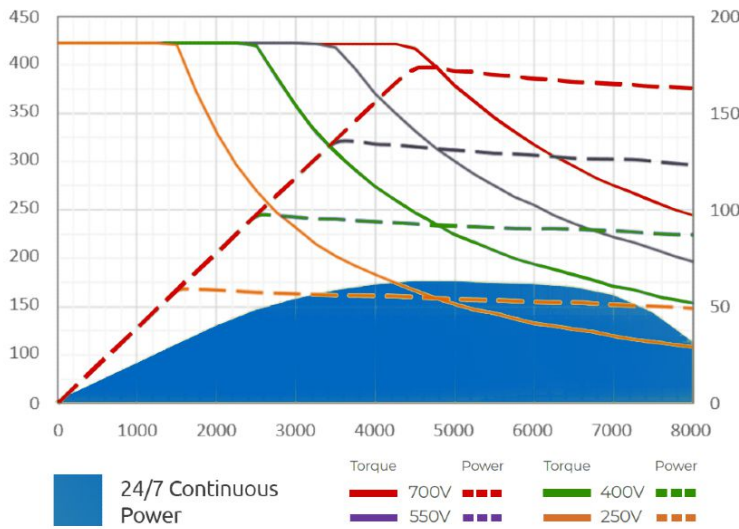
Example Electrical Performance with 800V controller @450ARMS F345-X
